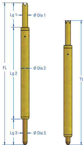
Single-Ended Probe
